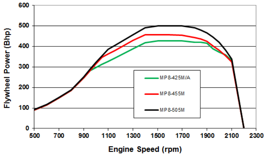
2017 MP8 Maxidyne Power Curves
