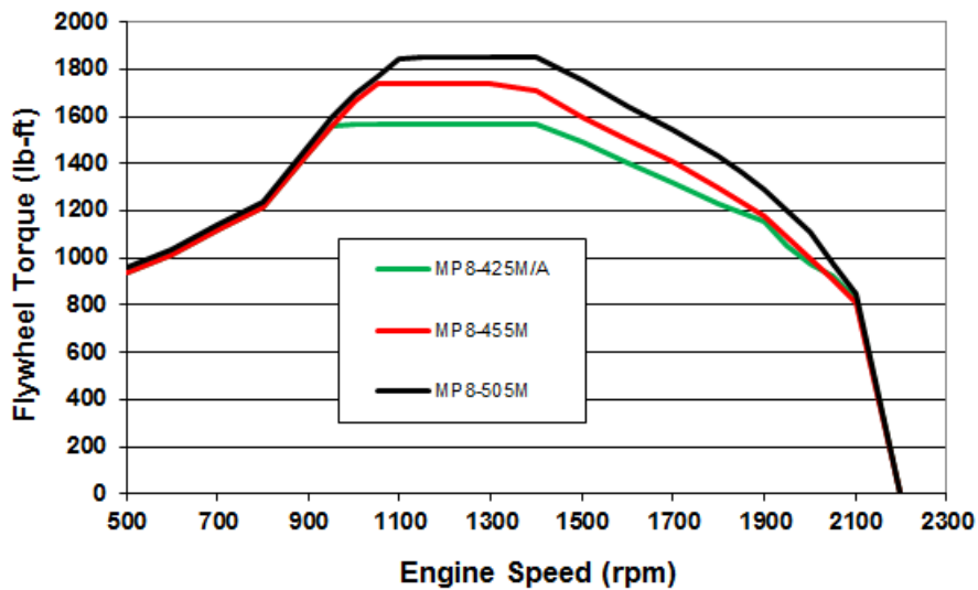
2017 MP8 Maxidyne Torque Curves
